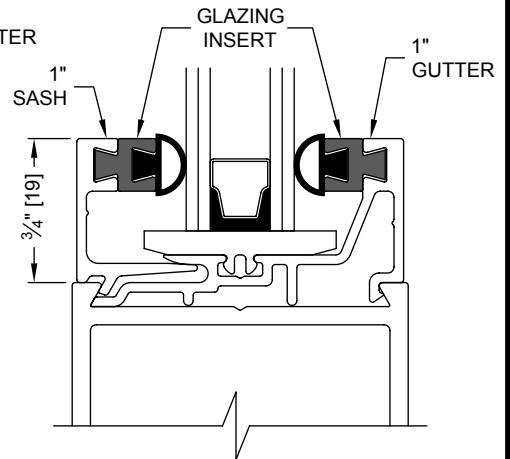
9/16" [14] GLAZING
