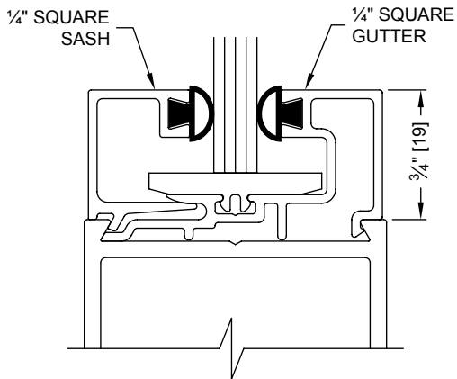
1/4" [6] GLAZING (STANDARD)
