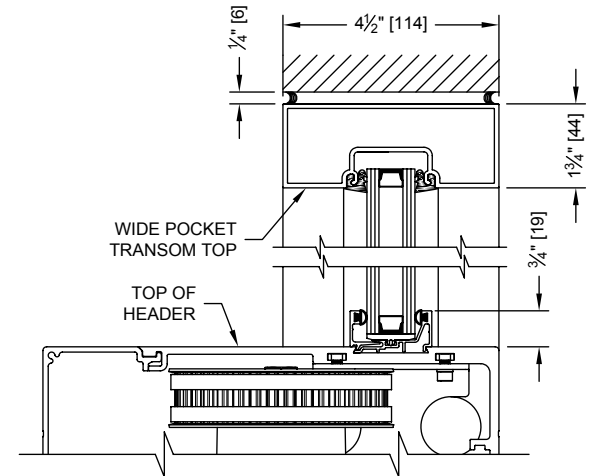
VERTICAL SECTION THROUGH TRANSOM (SHOWN WITH 1" THERMAL GLAZING)
