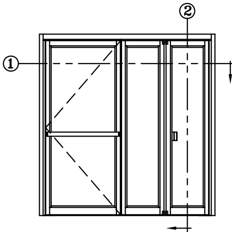
ELEVATION VIEW
