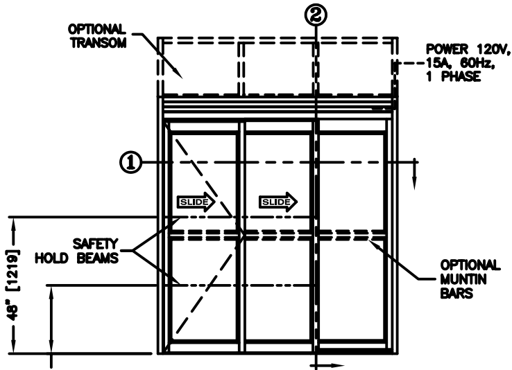
ELEVATION VIEW
